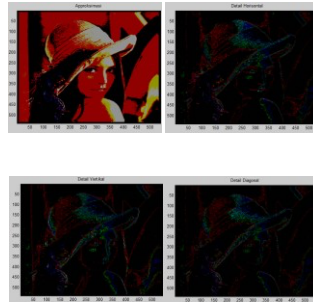
Figure IV-2. RGB image of Wavelet Decomposition "Lena.bmp"
